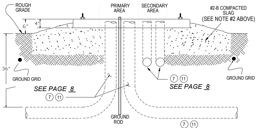
DETAIL "D"
