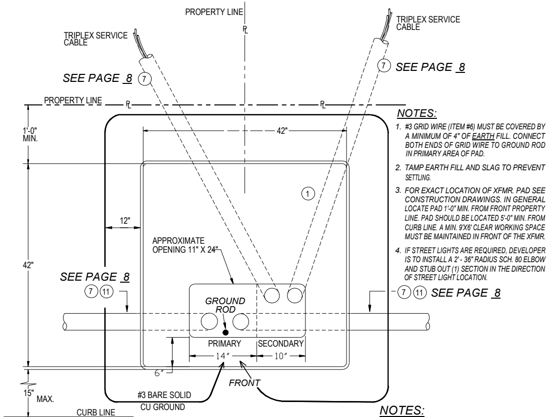
PLAN VIEW
