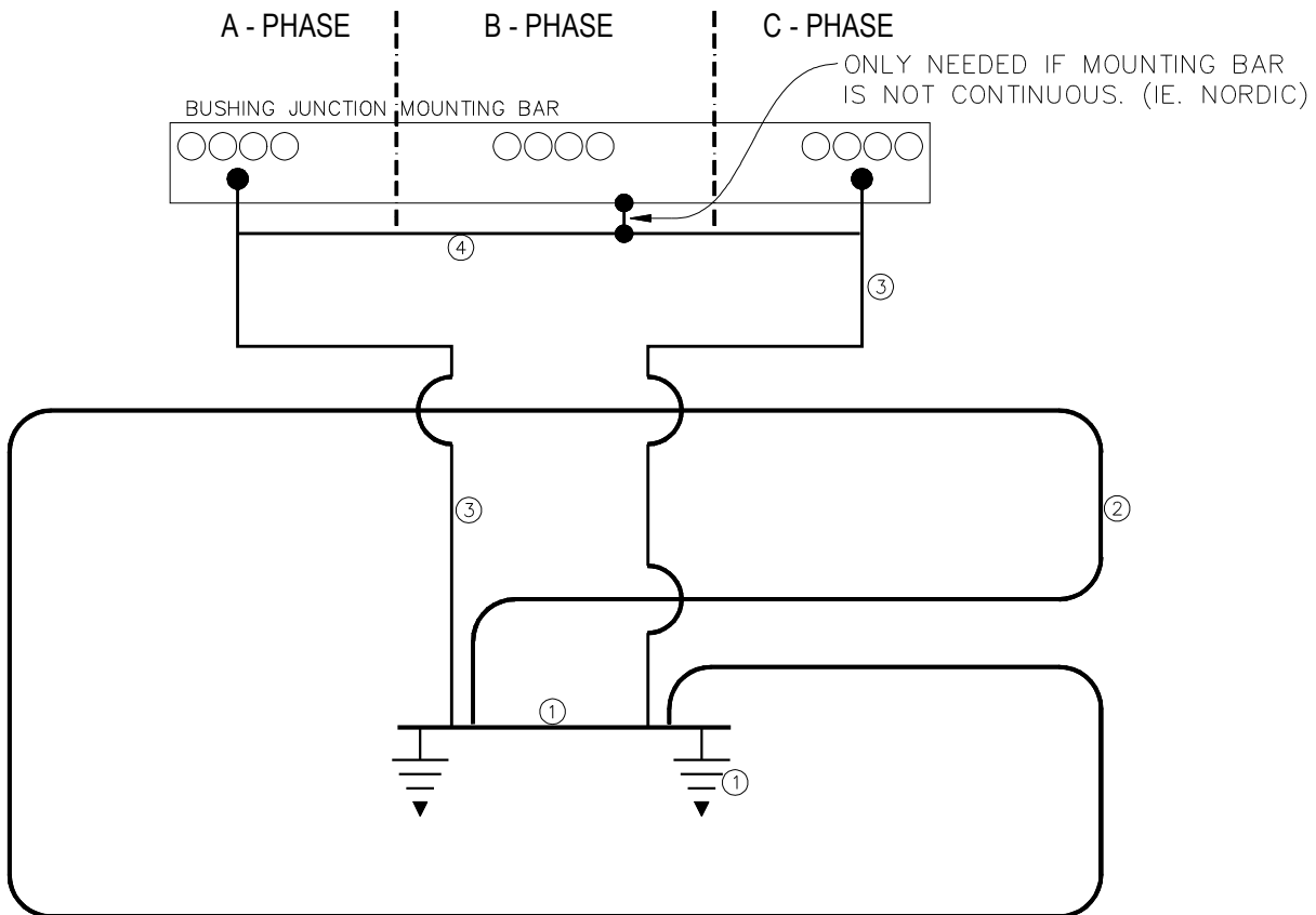
SECTIONALIZING ENCLOSURE GROUNDING SCHEMATIC
