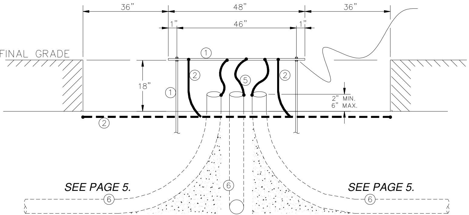
GROUND BUS DETAIL
