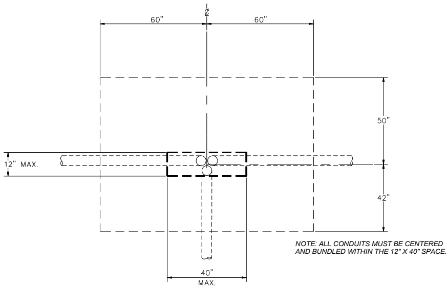
FRONT OF ENCLOSURE TYPICAL CONDUIT AND SWEEP PLACEMENT AREA FOR SECTIONALIZING ENCLOSURE. (8 BENDS MAX.)
